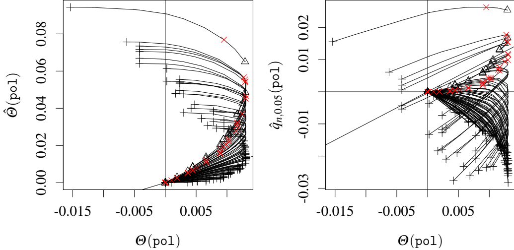
Figure 3: Max lower bound strategy. Graph of \Theta(\text{po1}) against \hat{\Theta}(\text{po1}) and \hat{q}_{n,0.05}(\text{po1}) . Each trajectory represents the change in those quantities when \eta varies. The cross corresponds to \eta = 0 , i.e., \text{po1} = \hat{\text{po1}}_1 . The triangles correspond to the end of the trajectory, i.e., \rho = q_{0.02} = -2.05 . The red X marks the quantities under the \hat{M}\hat{b}_{0.05} strategy. We plotted only the first 100 trajectories in order to have a readable output. In both plots, the first bisector, i.e., the y = x line, is drawn.
