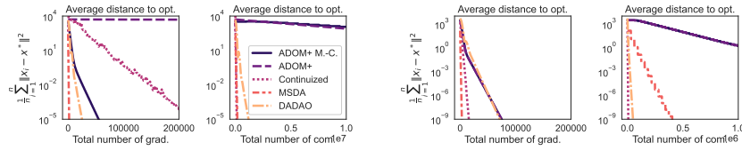
Figure 2: Comparison between ADOM+ [27], the continuized framework [12], MSDA [42] and DADAO, using the same data for the linear regression task, and the same graphs ( from left to right: line with n = 150 , complete with n = 250 ).
