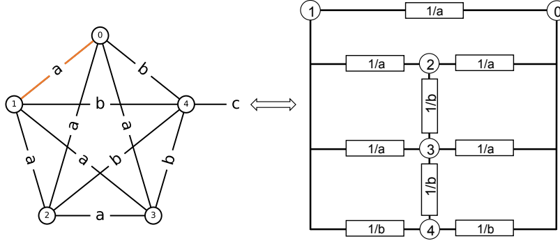
Figure 4: Equivalent resistance network if some current passes between node 0 and node 1 of the Barbell graph K_5 - K_5 . By symmetry of the resistance network, no current passes through the edges 2 – 3 and 3 – 4 and we have \frac{1}{2R_a} = a + \frac{2}{\frac{1}{a} + \frac{1}{a}} + \frac{1}{\frac{1}{b} + \frac{1}{b}} = 2a + \frac{b}{2} .
