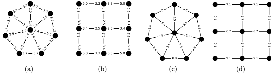
Figure 6: Optimal communication rates for the problem 83 obtained by solving the SDP from Prop. 4.1, under constraints \forall i, \sum_{j, (i,j) \in \mathcal{E}} \lambda_{ij} \leq 1 for (a,b) and \sum_{(i,j) \in \mathcal{E}} \lambda_{ij} \leq 1 for (c,d). For the sake of readability, we multiplied the values by 10 in (a,b), and by 100 in (c,d).
