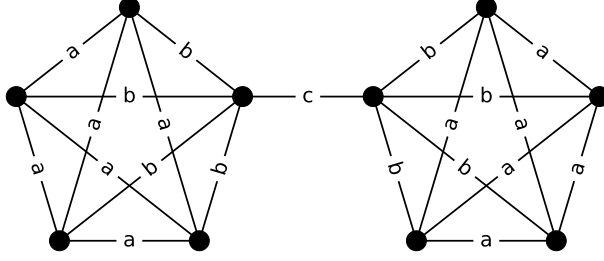
Figure 3: The barbell graph K_5 - K_5 .
