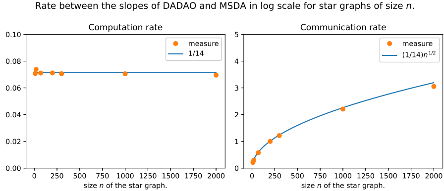
Figure 7: Rate between the slopes in log scale of DADAO and MSDA for star graphs of size n \in \{10, 20, 70, 200, 300, 1000, 2000\} .
