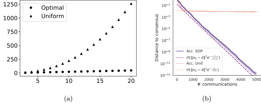
Figure 1: (a) Optimal value of \sqrt{2\chi_1\chi_2} for problem (5) under constraint \mathcal{C}_1 compared to the one obtained with uniform weights 1/|\mathcal{E}| , as a function of n for the barbell graph. (b) Convergence rate for the accelerated gossip procedure on a barbell graph K_{50} - K_{50} using both the edge weights given by our SDP and the uniform ones. For reference, we plot the theoretical rates, denoting by \chi_1^*, \chi_2^* the values obtained using the SDP weights, and by \chi_1, \chi_2 the ones obtained with 1/|\mathcal{E}| . Averaged over 20 runs.
