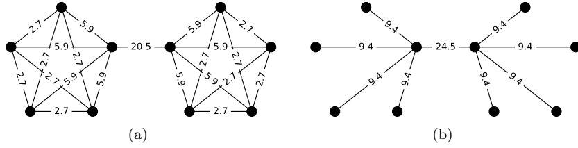
Figure 5: (a) Weights found by our SDP for the Barbell graph K_5 - K_5 , leading to \sqrt{\chi_1 \chi_2} \simeq 12.9 . (b) Optimal weights for the subgraph where edges a were removed, leading to a value of \sqrt{\chi_1 \chi_2} \simeq 10.2 . For the sake of readability, all values were multiplied by a factor of 100.
