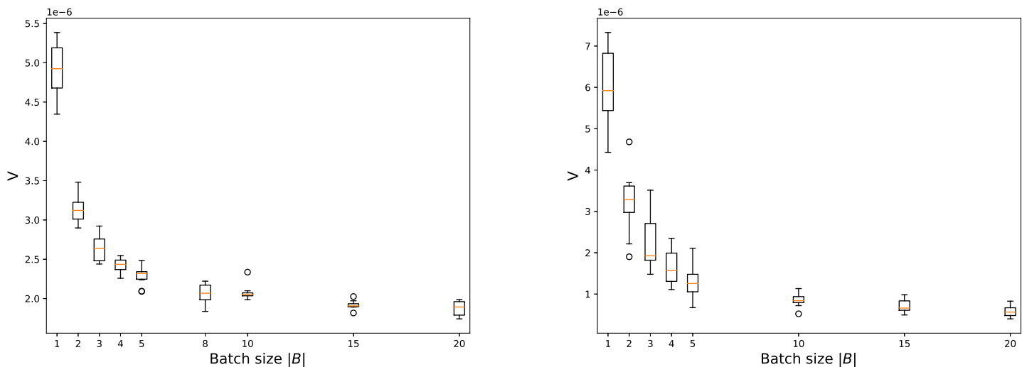
Figure 1: Variance \mathbf{V} reduction of the fluctuation process with increasing mini-batch size. Left: Regression task on simulated data. \mathbf{V} is an empirical estimation from 1000 realisations of the variance of \langle \|\cdot\|_2, \mu_t^N \rangle , where N = 800 and t = 1.25 . The other parameters are d = 40 , \alpha = 0.1 , \beta = 1 , and the noise is \varepsilon_k^i \sim \mathcal{N}(0, 0.01 I_d) . The boxplots are obtained with 10 samples of \mathbf{V} . Right: Classification task on MNIST dataset. \mathbf{V} is an empirical estimation from 30 realisations of the variance of \frac{1}{N} \sum_{j=1}^N W_k^{\mathbf{o},0,j} , where N = 10000 and k = 3000 ( t = 0.3 ). The boxplots are obtained with 10 samples of \mathbf{V} .
