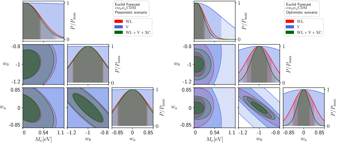
Fig. 9. Forecast contours for the w_0w_a CDM model, in the pessimistic ( left ) and in the optimistic ( right ) scenarios.
