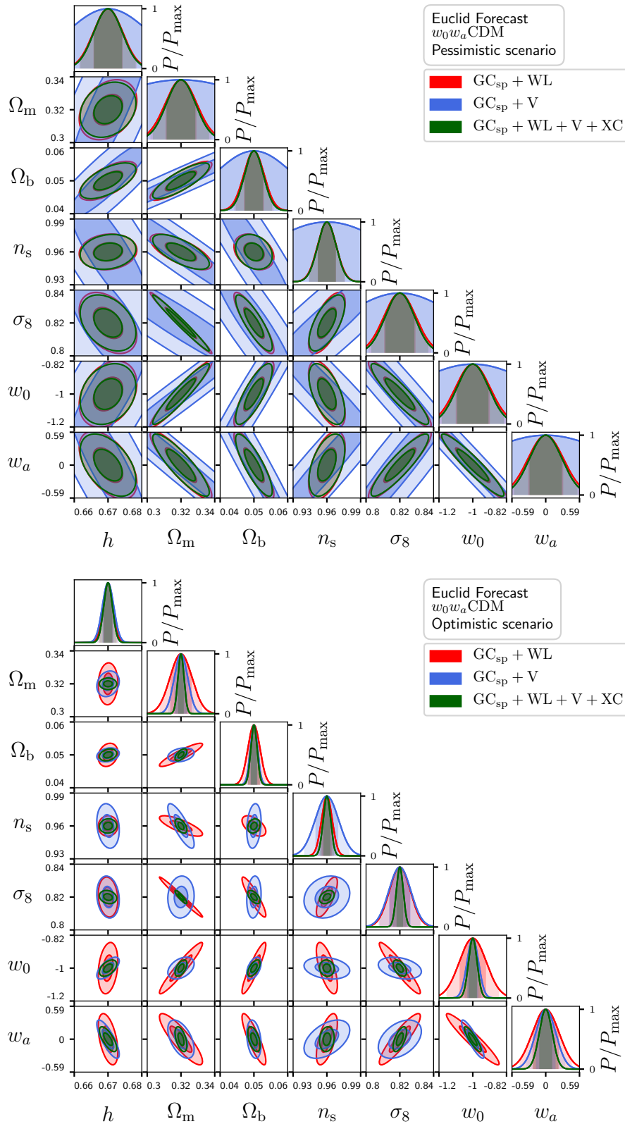
Fig. 7. Full contour plots when \text{GC}_{\text{sp}} is combined with WL + V + XC for the w_0w_a\text{CDM} model, in the pessimistic ( top ) and in the optimistic ( bottom ) scenarios.
