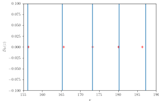
Figure 1: Comparison of \nu -zeros of D_\nu(z) for z = 23 with the asymptotic development (7)
