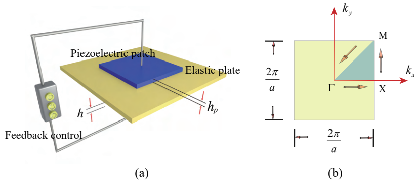
Figure 4: (a) Unit cell configuration (b) Irreducible first Brillouin zone
