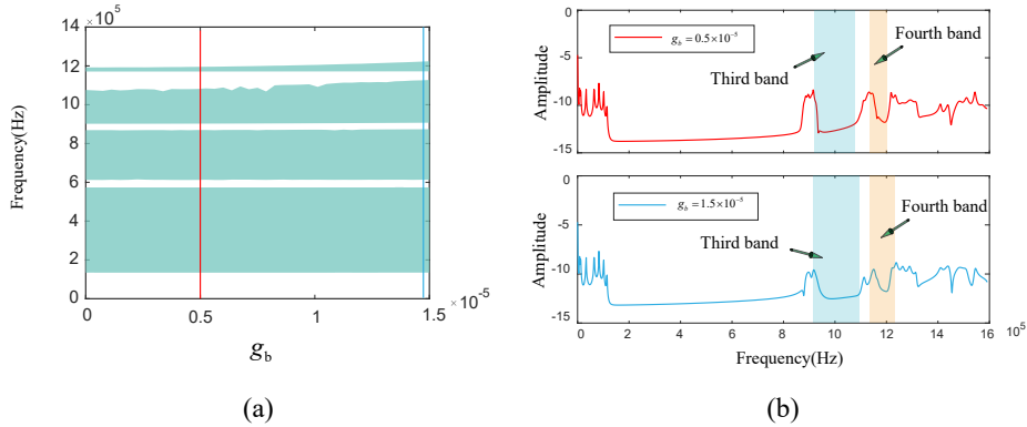
Figure 8: Effect of g_b on vibration control. (a) Evolution of the first four band gap frequency ranges with respect to g_b . (b) Dynamic response in frequency domain by considering two cases with g_b = 0.5 \times 10^{-5} and g_b = 1.5 \times 10^{-5} . Positions of the third and the fourth band gaps calculated in (a) for the two cases, are highlighted on (b) to provide comparison.
