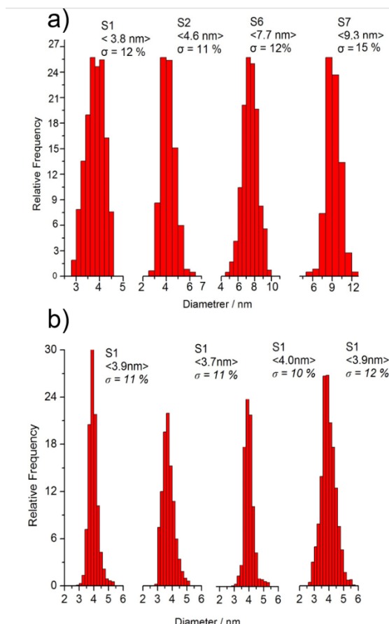
Figure 2. (a) Size distribution of Co NCs shown in the Fig. 1 (a-d) made at different bulk organic solvents. (b) Size distribution of Co NCs (sample S1) made up from several syntheses.
