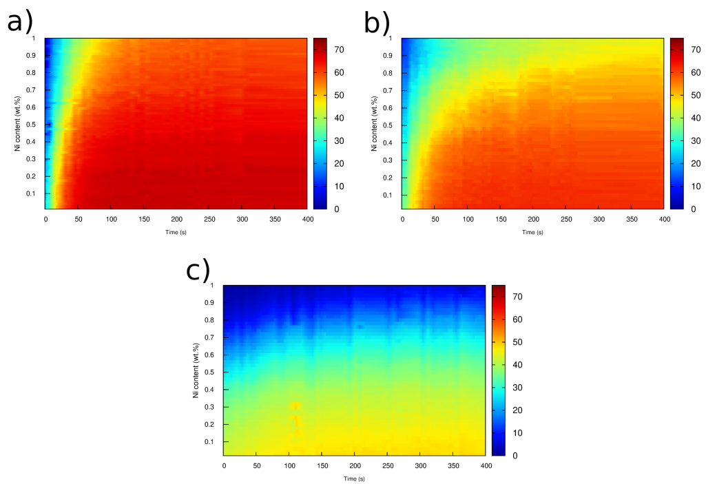
Figure S3: Heat maps illustrating ferrite volume fraction evolution as a function of time and nickel composition at : a) 730°C, b) 750°C and c) 775°C.
