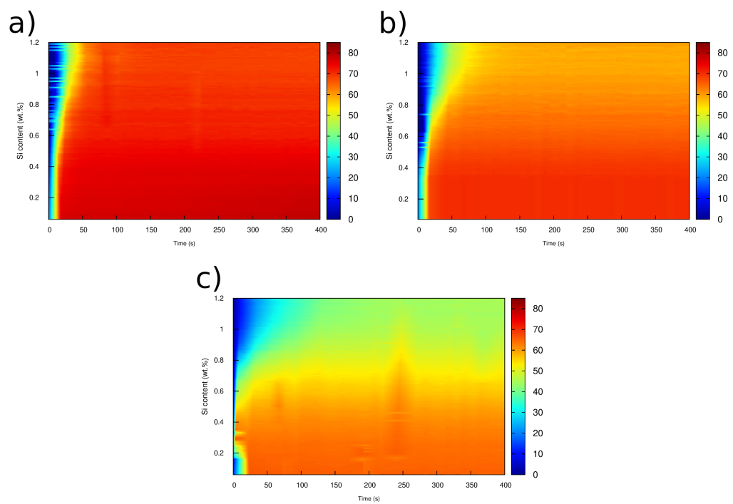
Figure S8: Heat maps illustrating ferrite volume fraction evolution as a function of time and silicon composition at : a) 730°C, b) 750°C and c) 775°C.
