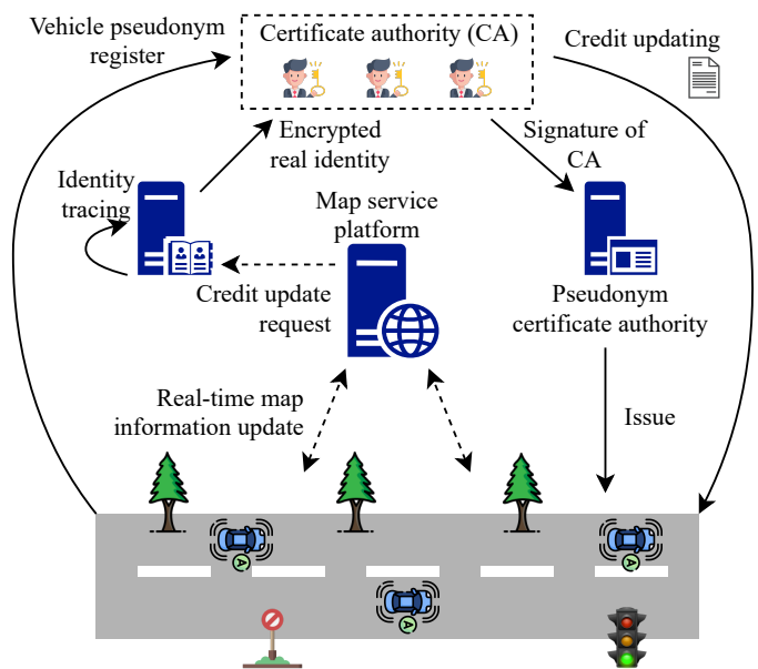
Fig. 6. System model with the SPIR scheme [121].
