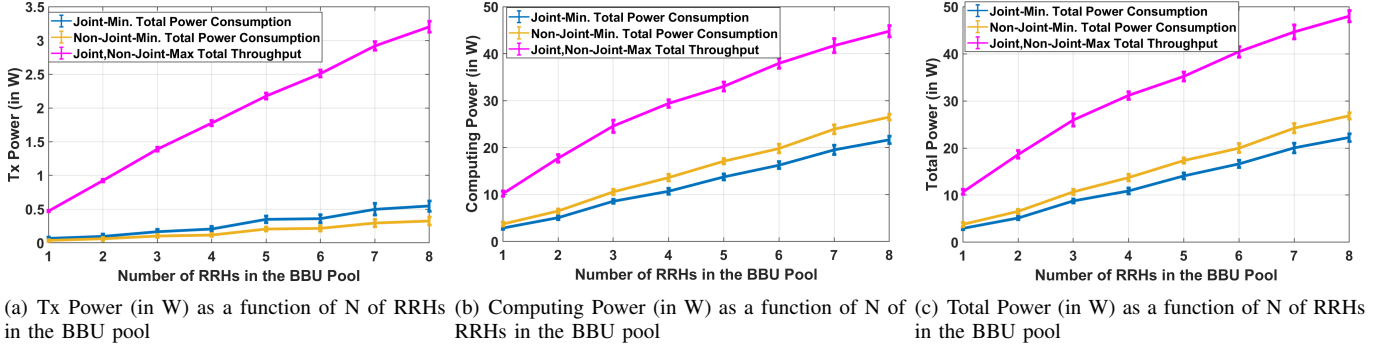
Fig. 1. Power Consumption
