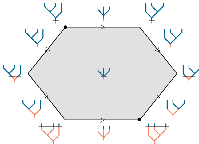
FIGURE 3. A 2-dimensional multiplihedron and the Tamari-type poset (CMT_3, <) on its oriented 1-skeleton.
