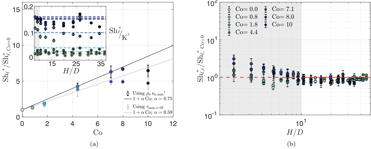
FIG. 4. (a) Evolution of the local erosion threshold values for Sh_\ell^* divided by the cohesionless threshold Sh_{\ell, Co=0}^* for H/D \gtrsim 10 using the maximum surface velocity (in black) and the maximum shear stress on the surface (in grey). The solid lines show a fit of the form Sh_\ell/Sh_{\ell, Co=0} = 1 + \alpha Co for cohesion numbers 0 \leq Co \leq 8 with \alpha = 0.75 \pm 0.04 (R-square: 0.9944) for the maximum local velocity and \alpha = 0.59 \pm 0.07 (R-square: 0.9653) using the maximum shear stress. Inset: Threshold values for Sh_\ell^* plateau for H/D \gtrsim 10 using the maximum surface velocity, and setting K = 1 . The colored dashed lines display the averages for a given Co number. (b) Local cohesive Shields number, Sh_{\ell,c}^* divided by the cohesionless local Shields number Sh_{\ell, Co=0}^* when varying the dimensionless distance H/D . The gray shaded area shows H/D \lesssim 10 , i.e. where the jet is not fully developed.
