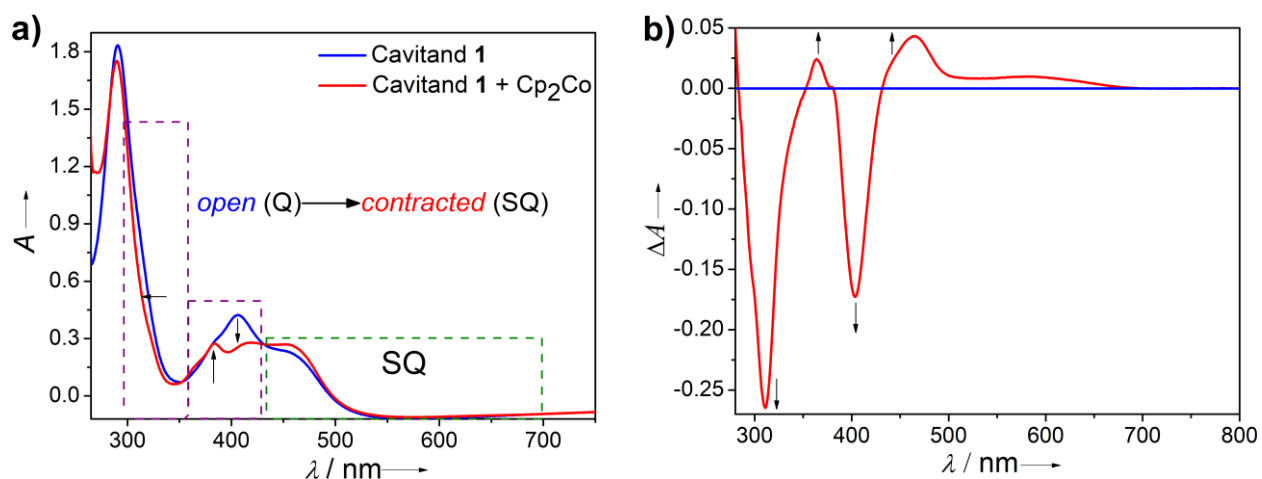
Fig. 6. (a) UV-Vis absorption of cavitand 1 before (blue) and after (red) addition of Cp 2 Co (1 μM solutions in DMF; 2 equiv. of Cp 2 Co) at T = 298 K with (b) the corresponding differential UV-Vis spectra. Green dashed box highlight the SQ formation while purple dashed boxes highlight the change in absorption due to conformational switching.
