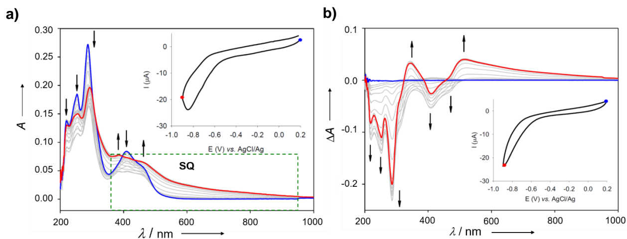
Fig. 5. (a) UV-Vis-NIR spectra upon electrochemical reduction of cavitand 1 in the potential region of the first reduction step in 0.1 M n -Bu 4 NPF 6 /CH 3 CN measured at T = 293 K with a scan rate of 0.01 \text{ V s}^{-1} and the corresponding (b) differential UV-Vis-NIR spectra. Insets shows the cyclic voltammograms and the potentials (colored circles) where the UV-Vis-NIR spectra were taken.
