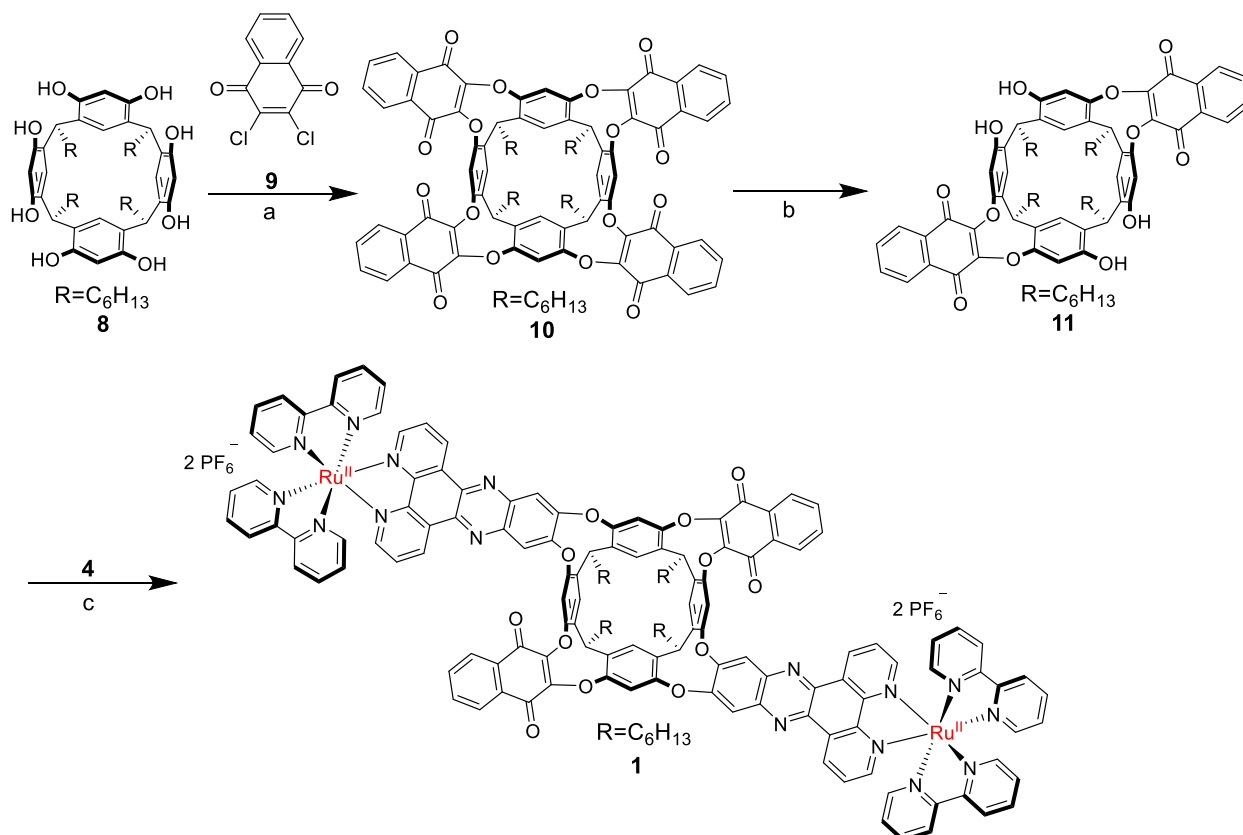
Scheme 2. Synthesis of cavitand 1 ; (a) \text{K}_2\text{CO}_3 , (\text{CH}_3)_2\text{SO} , 50\text{ }^\circ\text{C} , 16 h, 69%; (b) catechol, CsF, DMF, 70\text{ }^\circ\text{C} , 40 min, 35%; (c) 1) \text{Cs}_2\text{CO}_3 , DMF, 50\text{ }^\circ\text{C} , 5 h, 2) \text{KPF}_6 , \text{CH}_3\text{CN} , 23\text{ }^\circ\text{C} , 4 h, 37% (over two steps).
