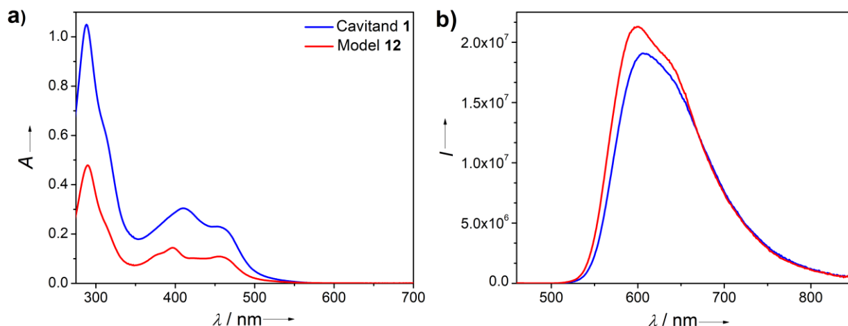
Fig. 4. a) UV-Vis absorption and b) emission spectra of cavitand 1 and model 12 ( 10^{-6} M solutions in \text{CH}_2\text{Cl}_2 ) at T = 298 K.
