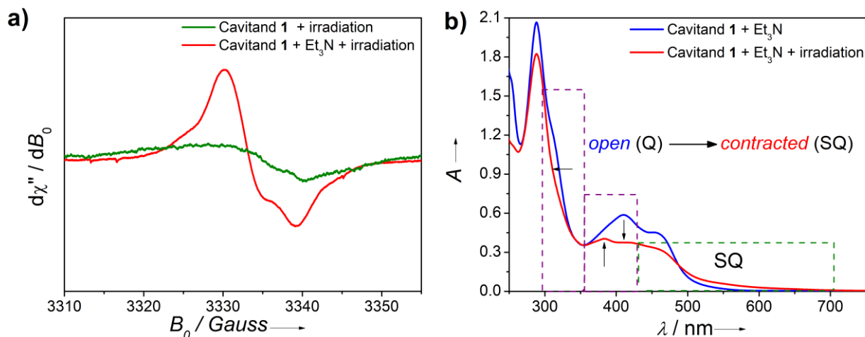
Fig. 7. Light-actuation of cavitand 1 in the solution of \text{CH}_2\text{Cl}_2 in presence of excess \text{Et}_3\text{N} (100 equiv.) as sacrificial electron donor. (a) EPR spectrum of 1 after irradiation with (red) and without (green) sacrificial donor at T = 120 K. (b) UV-Vis absorption spectra after 15 min of irradiation at 420 nm ( 10^{-6} M solutions in \text{CH}_2\text{Cl}_2 with 100 equiv. of \text{Et}_3\text{N} ) at T = 298 K. Green dashed box highlights the SQ formation (450–700 nm), while purple dashed boxes (300–350 nm) indicate the change in absorption due to conformational switching.
