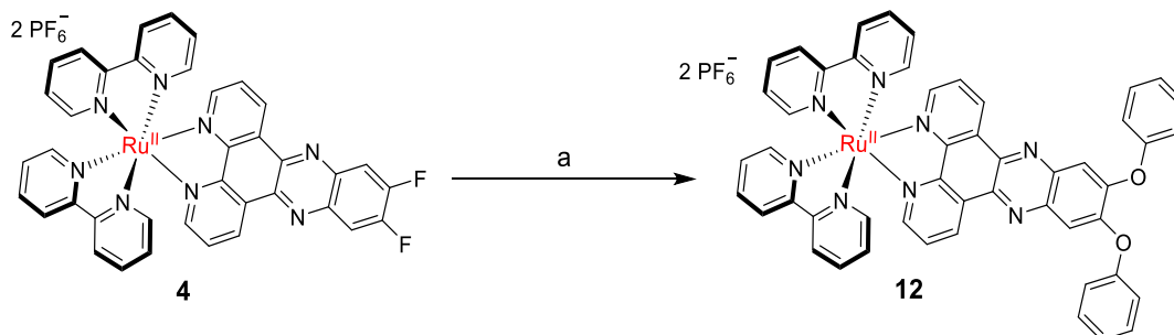
Scheme 3. Synthesis of model 12 ; (a) 1) Phenol, \text{Cs}_2\text{CO}_3 , DMF, 50\text{ }^\circ\text{C} , 5 h, 2) \text{KPF}_6 , \text{CH}_3\text{CN} , 23\text{ }^\circ\text{C} , 4 h, 97% (over two steps).
