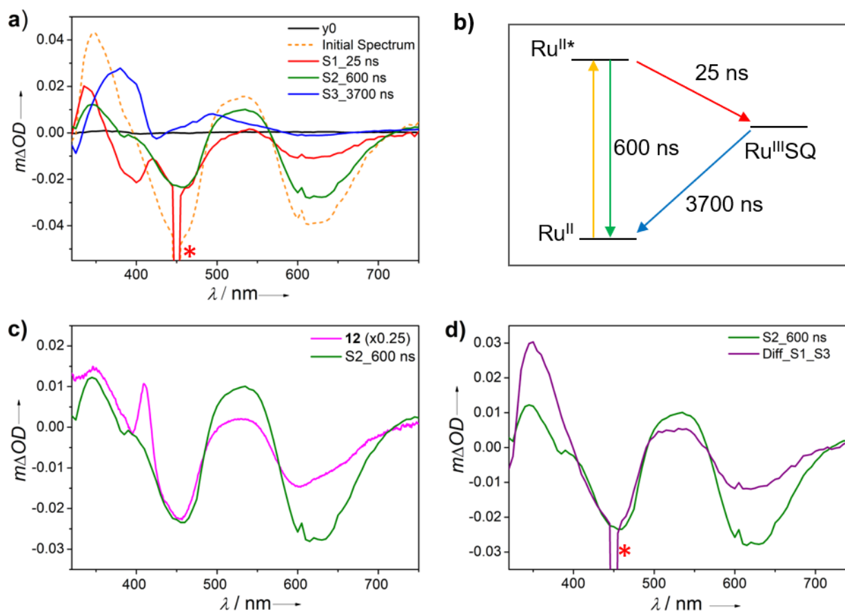
Fig. 8. (a) Species-associated decay spectra (SADS) obtained after excitation of cavitand 1 at 450 nm in degassed \text{CH}_2\text{Cl}_2 . The decay spectra were obtained by fitting the kinetic traces in a 20 \mu\text{s} time domain between 320 nm and 750 nm globally to a tri-exponential decay. (b) Schematic representation of the relevant photoexcited and charge-separated states which can be formed in cavitand 1 . (c) Comparison between SADS with 600 ns (green trace) and the transient absorption spectrum of the excited state of the reference complex 12 (pink trace). (d) Comparison between SADS with 600 ns (green trace) and a spectrum obtained by adding the SADS with 3700 ns (S3) to the 25 ns (S1) component (purple trace). The resulting spectrum corresponds well to the SADS of the species identified as S2, as shown in c). * Indicates stray light from laser excitation.
