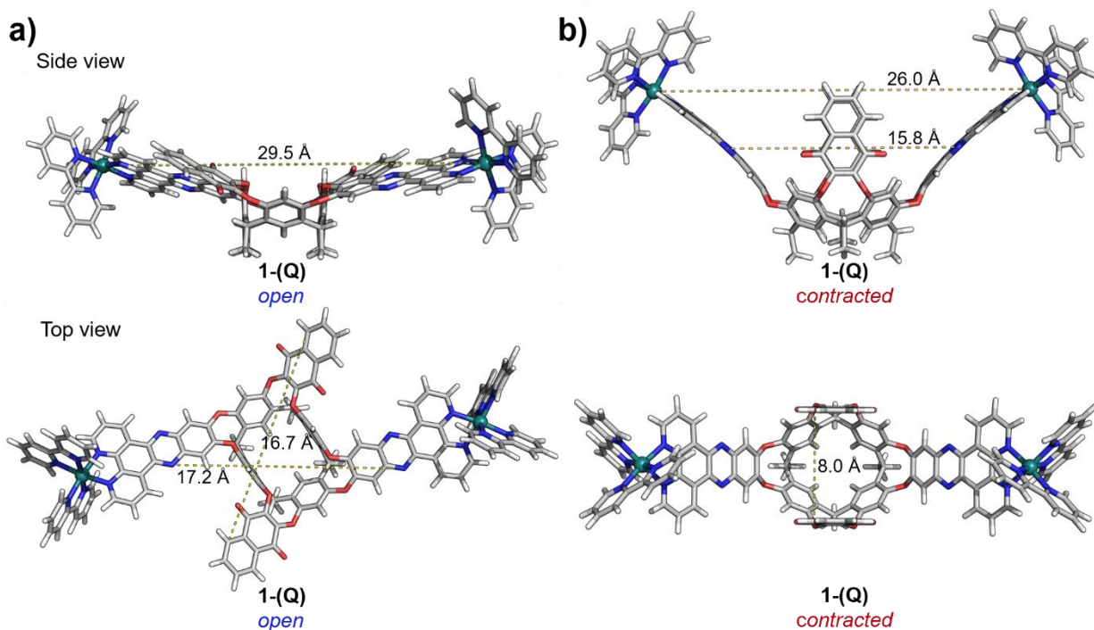
Fig. 2. Optimized geometries (DFT B3LYP/6-31G(d)) of cavitand 1 in a) open and b) contracted conformations in the Q state.
