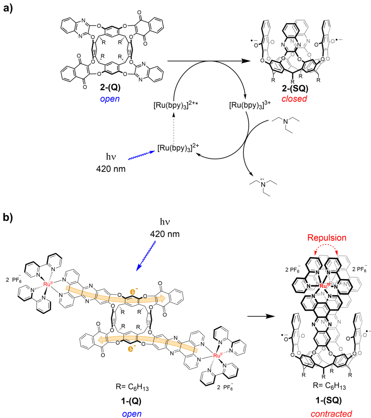
Fig. 1. a) Previously reported cavitand activated by intermolecular electron transfer. [13-14] b) Cavitand 1 activated by intramolecular electron transfer; the full closed conformation in the SQ cannot be achieved because of strong steric and electrostatic repulsion between the two Ru walls.
