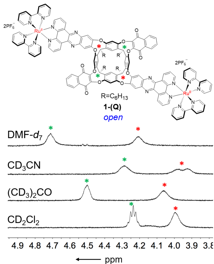
Fig. 3. Sections of the 1 H NMR spectra showing cavitant 1 ( c = 10^{-2} M, 300 MHz, T = 295 K) in the kite conformation in different solvents.
