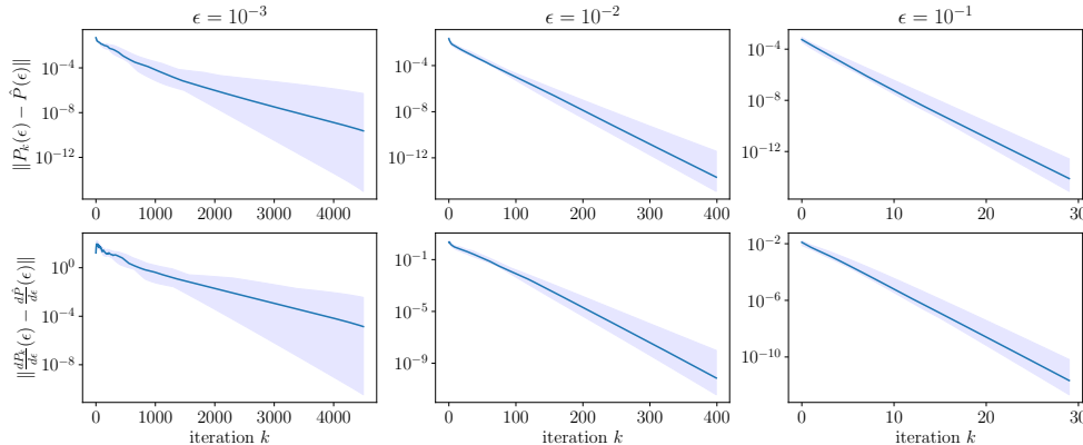
FIG. 2: Illustration of the linear convergence of the regularized transport plan P_k(\theta) (2.5) of Sinkhorn-Knopp ( SK_\theta ) (first line) and its derivatives \frac{dP_k}{d\theta}(\theta) (second line) towards the derivative of the entropic optimal transport problem ( OT_\theta ). Each column corresponds to a specific value of the regularization parameter: (left) \epsilon = 10^{-3} , (middle) \epsilon = 10^{-2} , (right) \epsilon = 10^{-1} .
