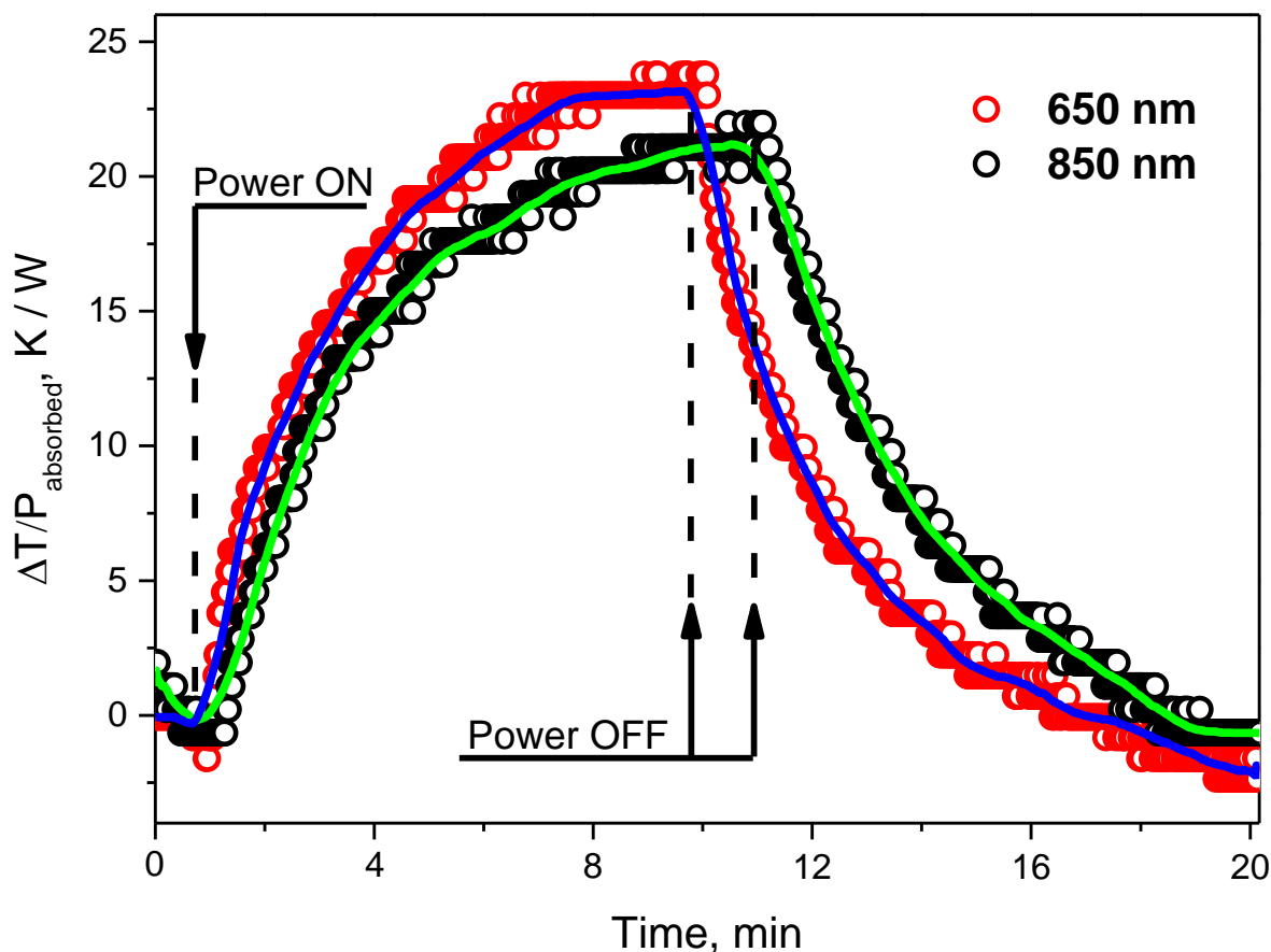
Figure 2. Photoinduced heating/cooling of colloidal solutions of O, N-CDs in water at two laser wavelengths: 650 and 850 nm. Open symbols correspond to experimental points and solid lines to exponential-like fitting curves.
