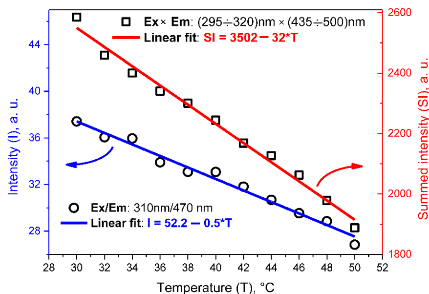
Figure 5. Temperature-dependent PL intensity of colloidal solutions of O, N-CDs in water (0.625 g/L). Black symbols—experimental points. Blue and red lines are linear fits of the experimental points corresponding, respectively, to a single spectral point Exc/Em: 310/470 nm and a spectral area: Exc × Em: (295–320) nm × (435–500) nm.
