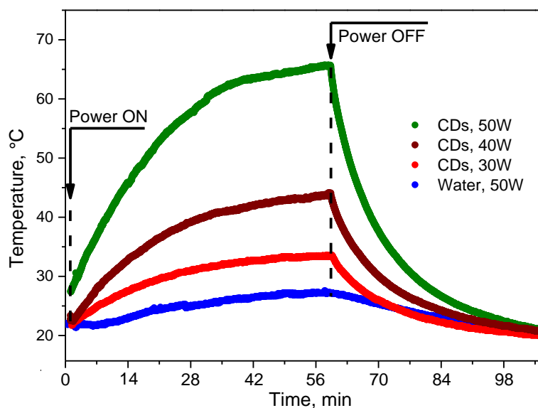
Figure 3. RF-induced heating/cooling of colloidal solutions of O, N-CDs in water at the RF generator powers of 50, 40, and 30 W and water at the RF generator power of 50 W.
