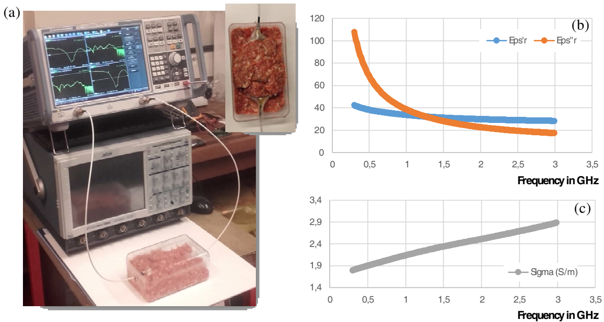
Figure 4. (a) Photograph of the measurement setup with the VNA when the antennae are buried in the meat. Characterization measurements of the used meat: (b) complex relative permittivity value in function of the frequency and (c) extraction of the conductivity value in S/m.
