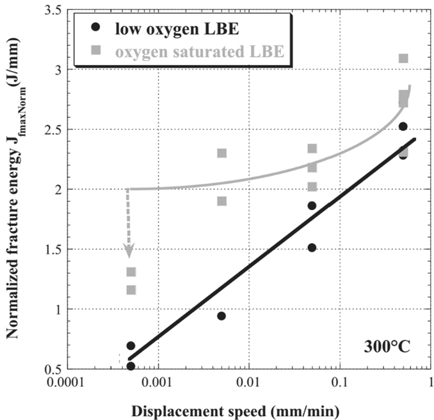
Fig. 4.24. Normalised fracture energy at F_{\max} as a function of the displacement speed and the LBE environment in terms of the dissolved oxygen concentration ( \text{SPT}^\dagger at 300^\circ\text{C} ) [504].
