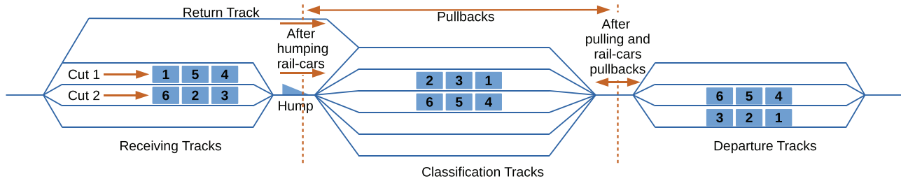
FIGURE 11 Three main steps of the sorting-by-train algorithm
