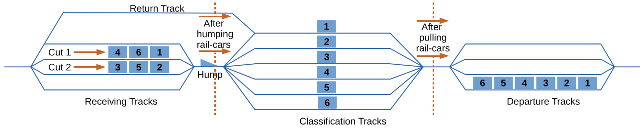
FIGURE 10 Three main steps of the sorting-by-block algorithm
