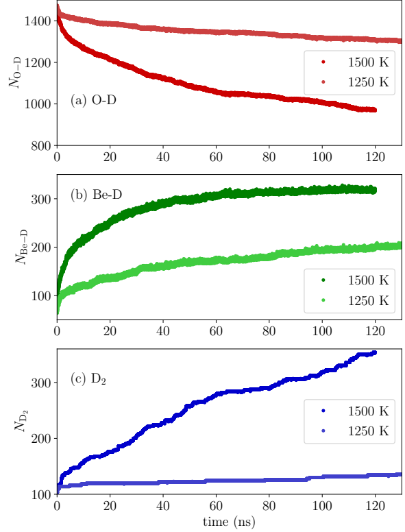
Figure 10: Total amount of D as O-D (a), Be-D (b) and D 2 (c) during the MD simulations at 1250 K and 1500 K.
