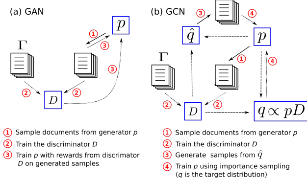
Figure 1. Training GANs vs GCNs. Solid arrows stand for sampling, dashed arrows depict dependence between distributions and dotted ones denote training. (a) Classical discrete GAN where: 1) the generator p samples sequences; 2) the discriminator D is updated according to these generated sequences and those from the training set \Gamma ; 3) the scores given by the discriminator D are used as reward in a policy gradient update of p . (b) Our GCN approach where \hat{q} and q respectively stand as the behavior and target distributions, which are defined by a cooperative scheme between D and p . After sampling from \hat{q} in 3), q is used in an importance sampling weight for the update of p in 4), which corresponds to the minimization of KL(q||p) . The distribution q is set as q(x) \propto p(x)D(x) to ensure convergence, and \hat{q} can take various forms, the closer to q the lower the variance.
