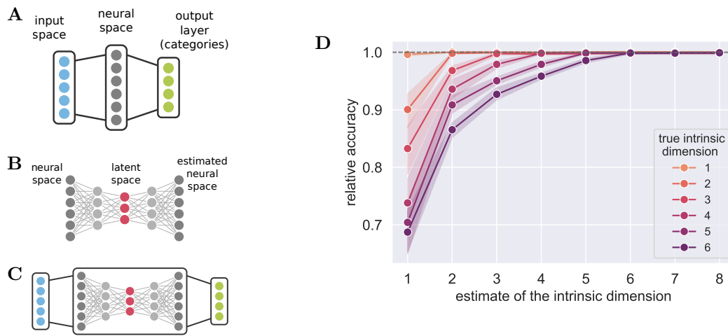
Figure 2: Description of the method use to probe the representation of a neural space. A neural network, (A), trained on a given classification task is then analyzed by using an autoencoder, (B), which is trained to reconstruct the neural activities under consideration. Using an hybrid network, (C), made of the original neural network and the activities predicted by the autoencoder, we then compute the classification accuracy on the test set (without any learning/finetuning). Varying the number of neurons in the bottleneck of the autoencoder serves as an estimate of the number of dimensions of the intrinsic space underlying the neural activities. (D) A simple example involving 10 Gaussian categories living in a controlled space of varying intrinsic dimension but same input dimension: when then number of dimensions in the reconstructed latent space reaches the true intrinsic dimension, the classification accuracy of the hybrid network (that forces the neural activities to be estimated through a small dimensional bottleneck) is the same as the one of the original network. The relative accuracy refers to accuracy of the hybrid network divided by the one of the original network (mean absolute accuracy is 71%). For each value of the true intrinsic dimension, the process is repeated for 10 trials, and error bars indicate 95% bootstrap confidence intervals.
