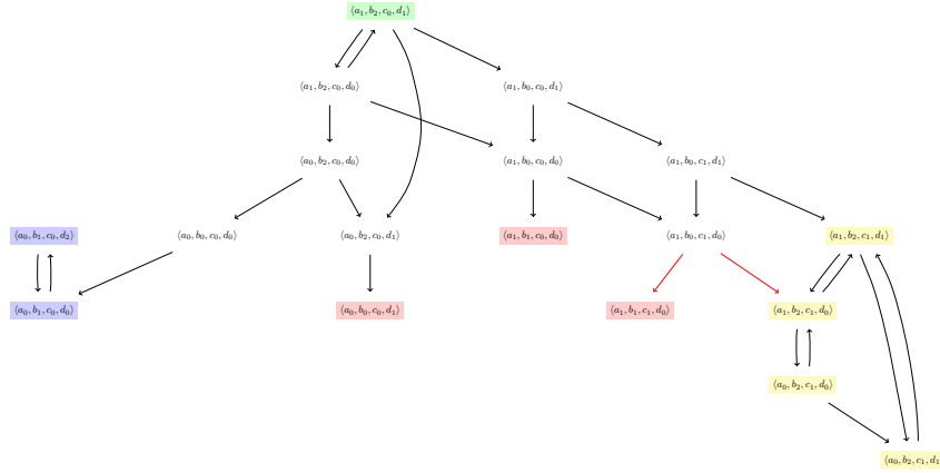
Figure 1.2: A part of the state-transition graph of the AAN given in Figure 1.1 for the asynchronous semantics, computed from the initial state: \langle a_1, b_2, c_0, d_1 \rangle until reaching attractors. We can observe three stable states: \langle a_1, b_1, c_1, d_0 \rangle , \langle a_1, b_1, c_0, d_0 \rangle and \langle a_0, b_0, c_0, d_1 \rangle ; an attractor of size 2: \{\langle a_0, b_1, c_0, d_0 \rangle, \langle a_0, b_1, c_0, d_1 \rangle\} (in blue) and an attractor of size 4: \{\langle a_1, b_2, c_1, d_1 \rangle, \langle a_0, b_2, c_1, d_1 \rangle, \langle a_0, b_2, c_1, d_0 \rangle, \langle a_1, b_2, c_1, d_0 \rangle\} (in yellow).
