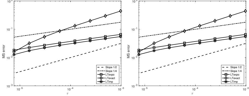
FIGURE 2. Mean-square errors as a function of the time step: Lie–Trotter splitting schemes: left ( \phi_\tau = \phi_\tau^L \circ \phi_\tau^{\text{NL}} ) and right ( \phi_\tau = \phi_\tau^{\text{NL}} \circ \phi_\tau^L ) ( \diamond for LTEXACT, \square for LTEXPO, \star for LTIMP). The dotted lines have slopes 1/2 and 1/4.
