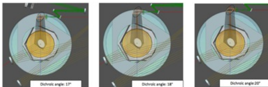
Figure 4. Footprint of the SCAO first mirror assembly on the MCAO LOR field of view for SCAO dichroic inclination angle values of 17°, 18° and 20°.
