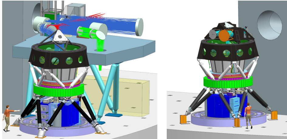
Figure 1. Left: MICADO and MAORY mounted together at the telescope. Right: MICADO at the telescope in its standalone configuration, i.e. with the SCAO module alone and a dedicated optical relay.
