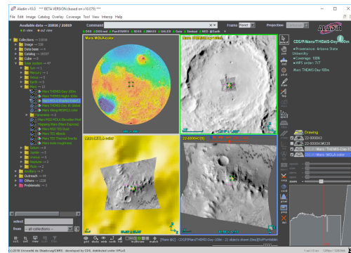
Fig. 2: CRISM spectral cube (georeferenced version converted to geofits) overlaid on MOLA and THEMIS multiresolution maps in Aladin.
