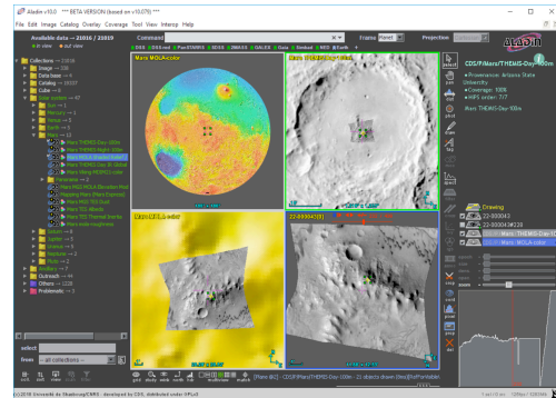
Fig. 2: CRISM spectral cube (georeferenced version converted to geofits) overlapped on MOLA and THEMIS multiresolution maps in Aladin.
