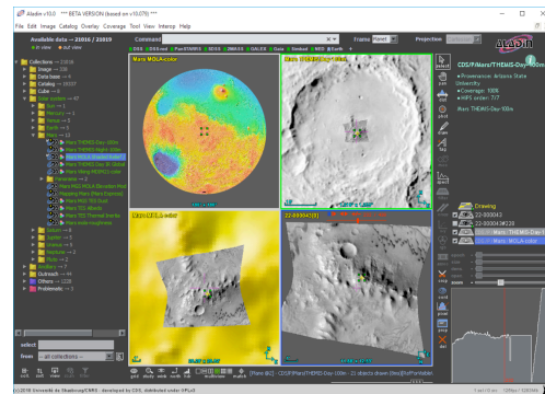
Fig. 2: CRISM spectral cube (georeferenced version converted to geofits) overlapped on MOLA and THEMIS multiresolution maps in Aladin.
