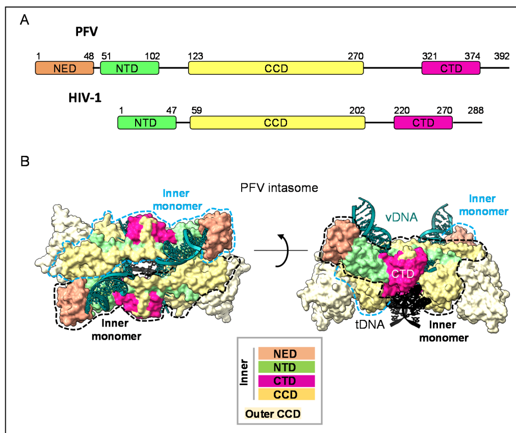
Figure 2. Domain organization of IN and structure of PFV intasome. (A) Integrase (IN) domains and interdomains are indicated by boxes and lines, respectively. Starting and ending amino acid residues are indicated above the boxes [30]. PFV integrase (upper representation) has an additional N-terminal extension domain (NED, in orange) that is not present in HIV-1 integrase (lower representation). N-terminal domain (NTD) is in green, the catalytic core domain (CCD) in yellow and C-terminal domain (CTD) in dark pink. This domain organization is conserved among retroviral integrases [2]. (B) Surface representation of the crystal structure (PDB: 3OS0, [27]) of PFV strand-transfer complex (STC) viewed along and perpendicular to the two-fold axis. IN is organized as an elongated tetramer along the DNA; the inner IN monomers are organized around vDNA and bring 3' extremities close to tDNA. The two inner monomers are outlined by dashed lines (light blue and black). The vDNA, tDNA and IN domains are indicated and follow the colour code of Figure 2A. Outer monomers are represented only by outer noncatalytic CCD domains, which are coloured in pale yellow.
