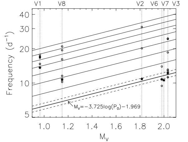
Fig. 8. Comparison between the observed frequencies in the BS stars and a period-luminosity relation for the fundamental mode of \delta Scuti stars (thick solid line) and for consecutive radial overtones (solid lines) based on theoretical frequency ratios from stellar oscillation models. The dashed lines indicate the 1\sigma error on the PLR and the vertical, dotted lines plots the M_V of the individual variables. The star-symbols indicate the frequency of highest amplitude in each star.
