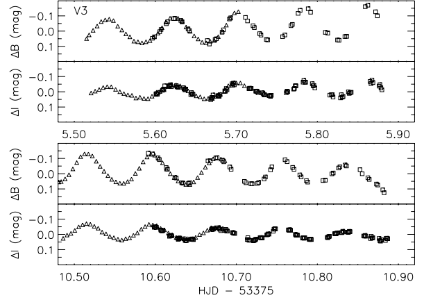
Fig. 2. Overlapping data on V3. Triangles are data from La Palma, squares are from La Silla. A slow trend with a frequency of 1.0 \text{ d}^{-1} was present in the La Silla B -data only, and was subtracted before merging the data (see Sects. 3.1 and 4.1).
