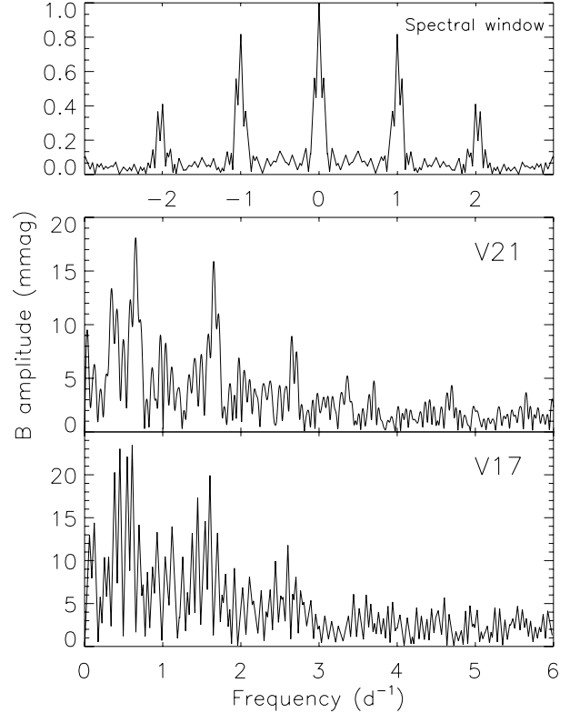
Fig. 10. Spectral window function and examples of amplitude spectra for two stars for which we detect long-period variability.
