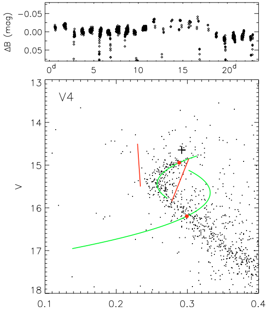
Fig. 16. 24-day light curve ( top ) and photometric solutions to the V4 binary system. The solid red lines are the \gamma Dor instability strip. The cross denotes the position of V4 in the CMD and the green curves are possible photometric solutions of the two components. The red dots mark a solution that puts both components on the cluster sequence.
