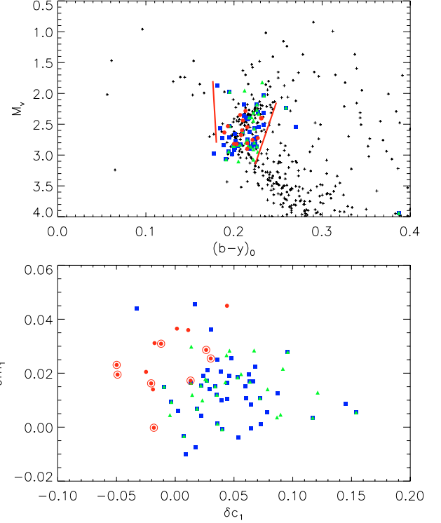
Fig. 12. Comparison of stellar parameters between the NGC 2506 \gamma Doradus stars and the known variables (Handler, private communication). The bona fide \gamma Doradus stars are shown as squares, the prime candidates as triangles, the NGC 2506 stars as filled circles, and the instability strip is from Handler & Shobbrook (2002). In the bottom panel, the multiperiodic (3 or more frequencies) NGC 2506 stars have been marked with an open circle as well.
