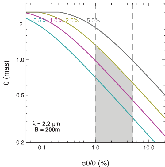
Fig. 2. Calibrator decision diagram (logarithmic scales) fixing the wavelength to 2.2 \mu\text{m} and the baseline to 200 \text{ m} : contours of the instrumental precision as a function of the diameter and diameter error of the calibrator. Stars below a given contour could be used at the labeled precision. Vertical dashed lines delimit the area corresponding to the typical diameter error obtained through (spectro-)photometric determinations (1–5%).
