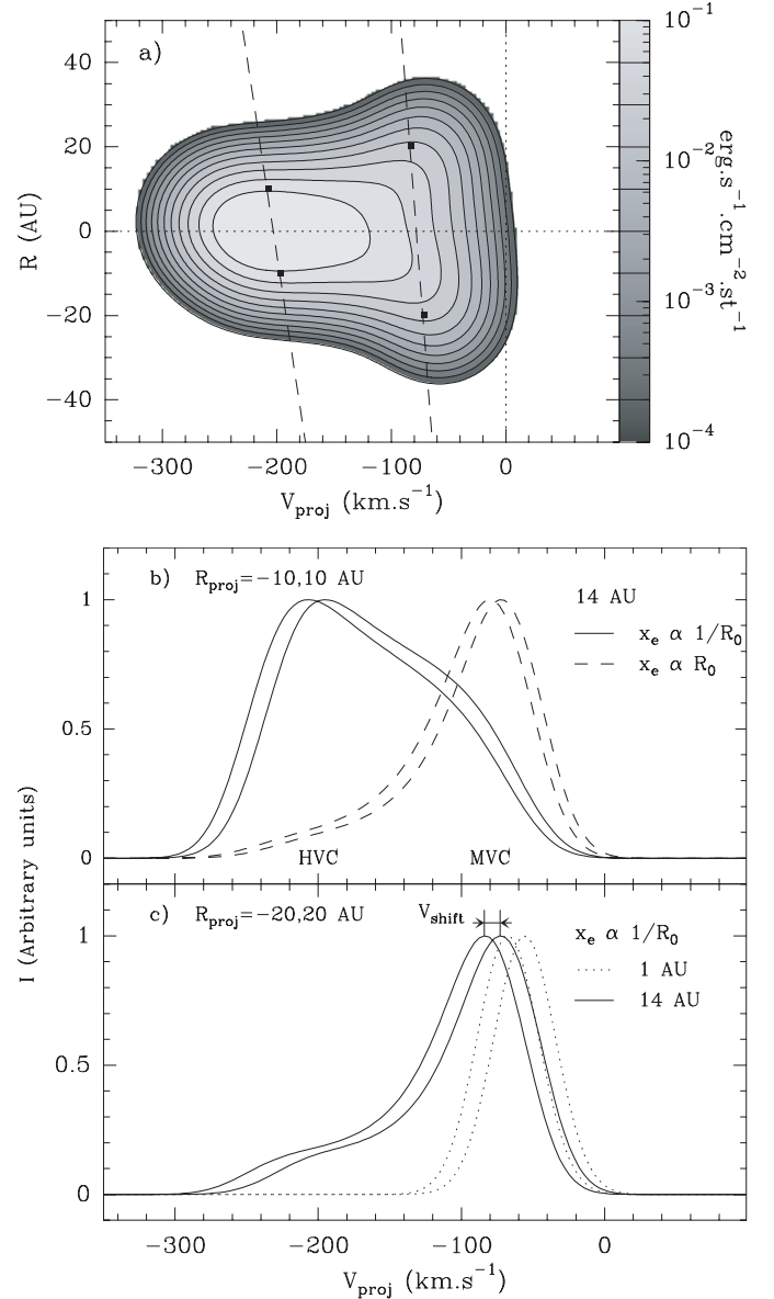
Fig. 2. a) Synthetic transverse Position-Velocity (PV) diagram for the warm solution (integrated over Z_{\text{proj}} = 50\text{--}60 AU) in the [O I] \lambda 6300 line, convolved with a 14 \text{ AU} \times 50 \text{ km s}^{-1} beam. i = 45^\circ and x_e = 0.1 \times (0.1 \text{ AU}/R_0) . Dashed lines are indicative of peak velocity shifts at 10 and 20 AU from the jet axis. b) Velocity profiles extracted from PV diagrams at R_{\text{proj}} = \pm 10 AU, convolved with a spatial beam of 14 AU for x_e = 0.1 \times (0.1 \text{ AU}/R_0) (solid lines) and x_e = 0.1 \times (R_0/1 \text{ AU}) (dashed lines), c) and at R_{\text{proj}} = \pm 20 AU, with spatial beams of 1 (dotted) and 14 AU (solid) for x_e = 0.1 \times (0.1 \text{ AU}/R_0) .
