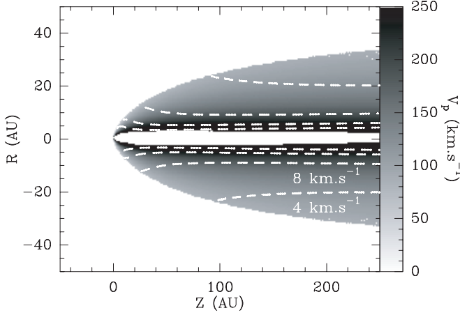
Fig. 1. Velocity components ( V_p, V_\phi ) in the (R, Z) plane for the warm solution ( \lambda = 13 ). Dashed lines: V_\phi varying from 4 to 16 \text{km s}^{-1} by steps of 4 \text{km s}^{-1} . Greyscale: V_p .
