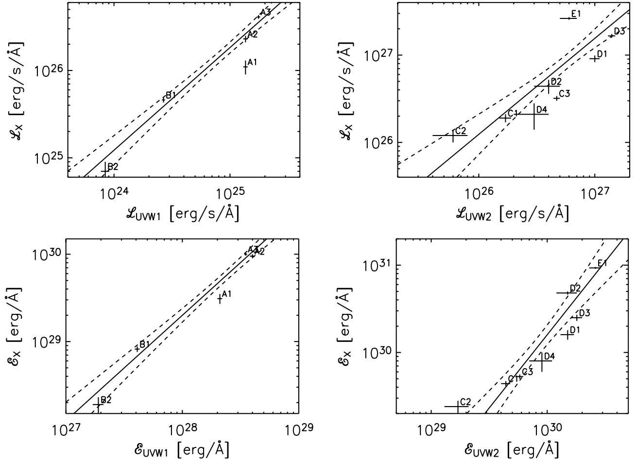
Fig. 3. X-ray vs. UV flare relationships. The two panels on the left use the UVW1 , the ones on the right the UVW2 filter. The upper panels are for the luminosity increase, the lower panels for the flare energy. Used throughout for the regression are spectral luminosity density and spectral energy density, as defined in Sect. 3.2. The crosses denote the flares, their sizes corresponding to the 1\sigma error. They are labelled according to their identification as in Figs. 1 and 2. The solid line in the plot indicates the best fit power-law regression. The flares have been weighted with their individual errors for the regression. The dashed lines contour the 3\sigma error, where \sigma is the standard deviation of the mean. The regression values are given in Table 2.
