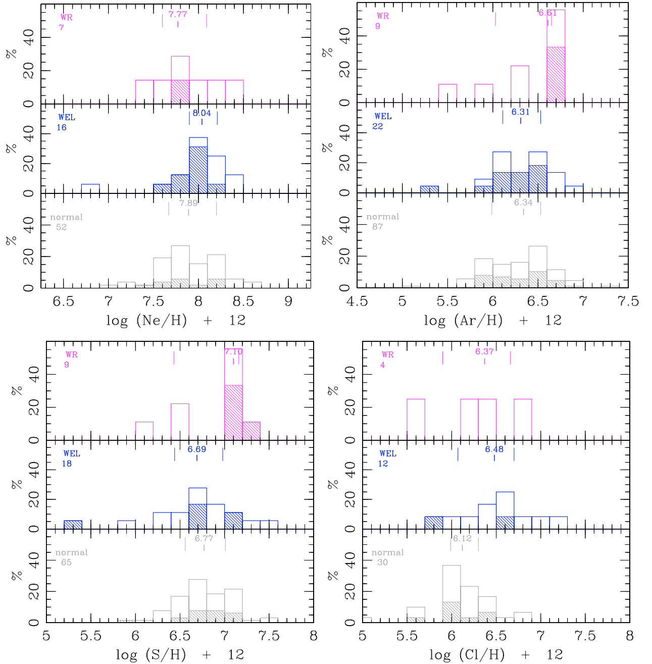
Fig. 20. Distributions of neon, argon, sulfur and chlorine abundance for Galactic bulge [WR], WEL and normal PNe. The same notation as in Fig. 13.
