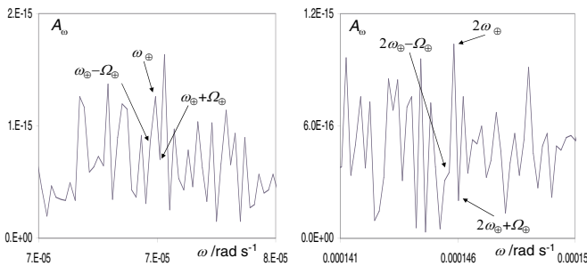
FIG. 3 (color online). Fitted Amplitudes A_{\omega} for a range of frequencies around the six frequencies \omega_i of interest (indicated by arrows).
