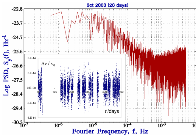
FIG. 1 (color online). Relative frequency difference between the CSO and the H-maser after removal of a linear fit per data set. Complete data (inset) and PSD of the longest data set.
