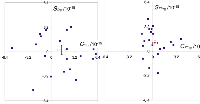
FIG. 2 (color online). Fitted sine and cosine amplitudes at \omega_{\oplus} and 2\omega_{\oplus} for each data set (squares) and the complete data (diamonds, with statistical errors). For clarity the error bars of the individual data sets have been omitted.
