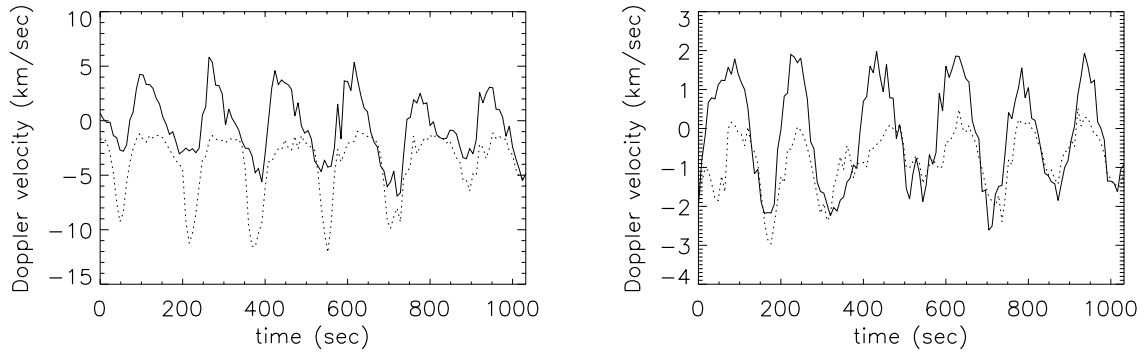
Fig. 3. Time evolution of the Doppler velocity for the UF No.1 of Fig. 2 ( left panel ) and for the calmest umbral position ( right panel ). Solid line represents the H\alpha Doppler velocity at \pm 0.29 \text{ \AA} , while dotted represents the \text{Ca II } 8542 \text{ \AA} Doppler velocity at \pm 0.09 \text{ \AA} . Positive Doppler velocities represent upward motion. We point out that the Doppler velocity scales of the two plots are different and that the calmest umbral position Doppler velocity amplitudes are smaller than the UF ones.
