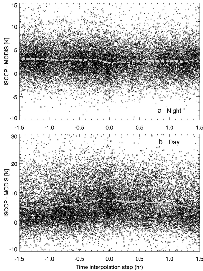
Figure 7. ISCCP-MODIS LST differences as a function of \Delta t_{MODIS-ISCCP} (as defined in the text) for (a) night and (b) day, for July 2003. The dashed lines mark the averages (at 4.5-min increments).
