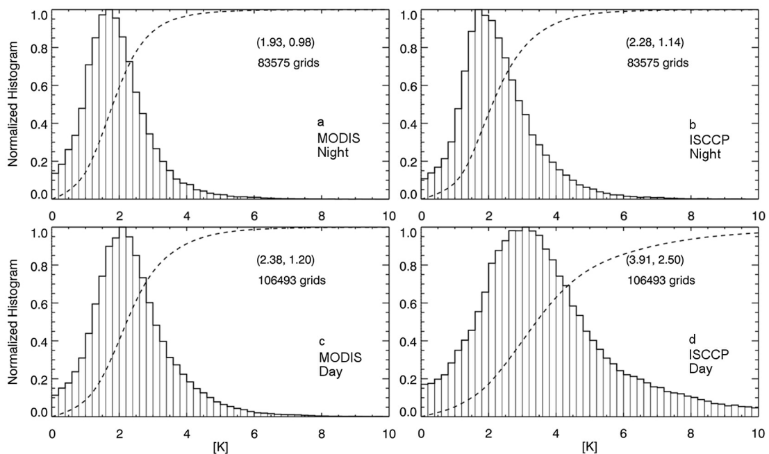
Figure 5. Histograms of standard deviations of LST from (a and c) MODIS and (b and d) ISCCP for night (Figures 5a and 5b) and day (Figures 5c and 5d) measurements for July 2003. The mean and standard deviation are in parentheses.
