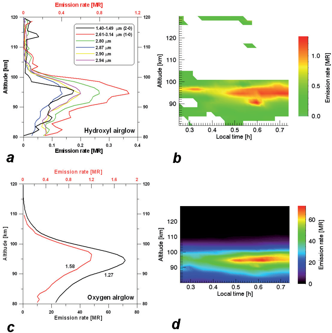
Fig. 2. Limb vertical profiles of the O 2 and OH nightglow emissions versus tangent altitude. Panel a ): vertical profiles of the OH emission at 2.80 μm (green), 2.87 μm (blue), 2.90 μm (yellow), 2.94 μm (magenta), plus all of these integrated from 2.61 to 3.14 μm (shown in red, only this one corresponding to the x axis on top in the same color, all the others refer to the bottom axis) and from 1.40 to 1.49 μm (black). Panel b ): the local distribution of the integrated bands (red curve of panel a ) versus local time and tangent altitude of the closest point of the tangent limb to the planet. It can be seen that the distribution of the OH emission varies even within a single orbit. For comparison, the O 2 emission at 1.27 (black, bottom axis) and 1.58 μm (red, upper axis) is shown for the same orbit in panel c ), and its variability in panel d ). In all cases the instantaneous geometrical vertical resolution from the distance of 10 800 km to 13 700 is better than 3.5 km. In order to improve the signal to noise ratio, pixels are averaged over the latitude range 10–35° N and all profiles are smoothed with a step of 2 km in height.
