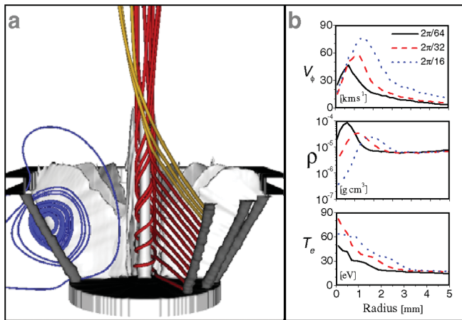
FIG. 5 (color). Results of MHD simulations. (a) Isodensity surfaces at 270 ns show the dense plasma around the wires ( 10^{-3} g/cm 3 , dark gray) and plasma streams ( 2.5 \times 10^{-5} g/cm 3 , light gray); streamlines from one of the wires are shown with the oppositely rotating flows separated visually by red and orange streamlines; the azimuthally averaged poloidal magnetic field lines are shown in blue. (b) Azimuthally averaged profiles of azimuthal velocity, density, and temperature taken 6 mm above the cathode at 200 ns.
