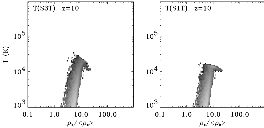
Fig. 11. Baryonic mass fraction at z = 10 per interval of the baryonic density contrast and per interval of the bulk temperature in the S_{3T} simulation ( left panel ) and per interval of gas temperature in the S_{1T} simulation ( right panel ), both simulations including photoionization processes.
