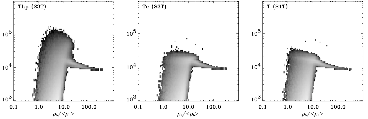
Fig. 5. Baryonic mass fraction at z = 5 per interval of baryonic density contrast and per interval of heavy particle temperature ( left panel ), per interval of electron temperature ( middle panel ) in the S_{3T} simulation, per interval of gas temperature in the S_{1T} simulation ( right panel ), light grey is high mass fractions and temperature is shown on the ordinate axis.
