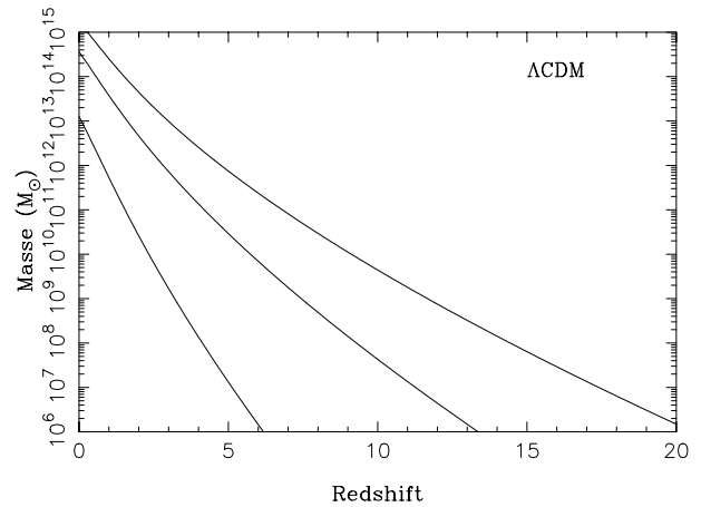
Fig. 12. Collapsing redshift and mass of (1-2-3)\sigma fluctuations (from left to right), computed by a spherical top-hat collapse model (Eq. (34)) in a \Lambda -cold dark matter universe.
