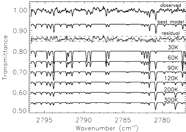
Fig. 2. Observed spectrum of W33A divided by the estimated local dust continuum to provide a transmittance spectrum, and model absorption spectra of \text{H}_2\text{CO} at various excitation temperatures, for N(\text{H}_2\text{CO}) = 2. \times 10^{16} \text{ cm}^{-2} . The best fit (see text) model spectrum and its residuals are shown just below the observed spectrum.
