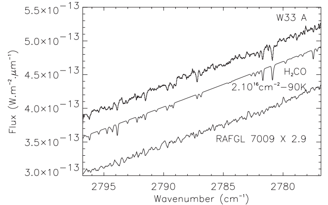
Fig. 1. UKIRT spectra of W33A and RAFGL 7009S compared to a gas phase \text{H}_2\text{CO} modelled spectrum multiplied by the estimated continuum of W33A and slightly shifted down for clarity.
