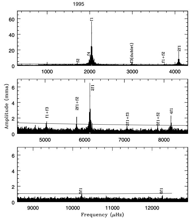
Figure 1. Weighted Fourier transform for 1995 data. The weights are the inverse square of the dispersion in each light curve. The line is the detection limit obtained from the Monte Carlo Simulation. Note the change in the y-axis for the lower panels.
