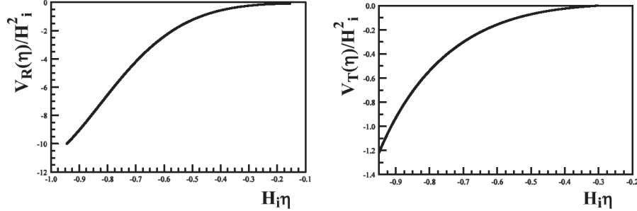
FIG. 2. The potentials \mathcal{V}_R(\eta)/H_i^2 (left panel) and \mathcal{V}_T(\eta)/H_i^2 (right panel) felt by curvature and tensor perturbations, respectively, vs H_i\eta , H_i being the Hubble parameter during the slow roll stage (see Fig. 3).
