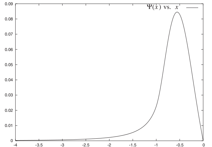
FIG. 5. The odd function \Psi(x) vs x for negative x [see Eq. (5.20)]. This function convoluted with the potential \mathcal{V}(\eta) yields the change on the quadrupole \frac{\Delta C_2}{C_2} [see Eq. (5.19)].
