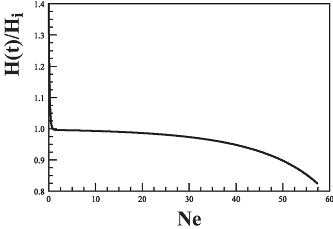
FIG. 3. H(t)/H_i vs the number of e-folds.
