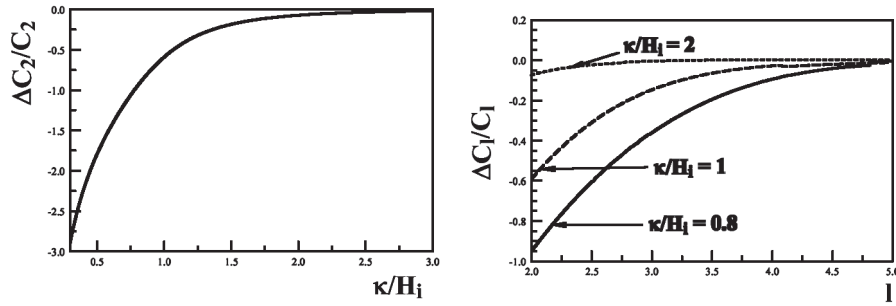
FIG. 4. \Delta C_2/C_2 vs \kappa/H_i (left panel) and \Delta C_l/C_l vs l for \kappa/H_i = 0.8, 1, 2 , respectively, for curvature perturbations, \kappa = a_0 H_0/3.3 .
