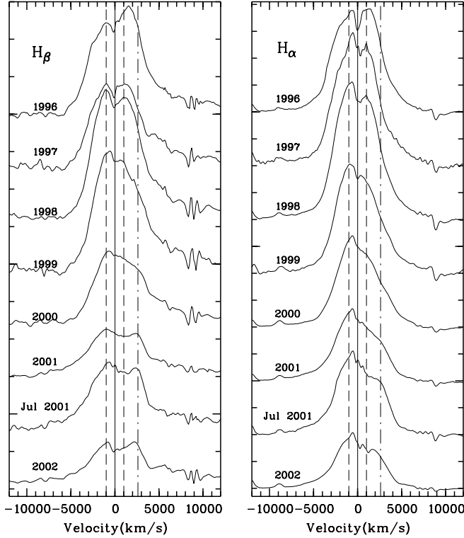
Fig. 6. Annual averages from 1996 to 2002 of the observed profiles of H \beta broad emission component after subtraction of the continuum and the narrow components of H \beta and [O III] \lambda\lambda 4959, 5007 ( left ). The same for H \alpha after subtraction of the continuum and the narrow components of H \alpha , [N II] \lambda\lambda 6548, 6584 and [S II] \lambda\lambda 6717, 6731 ( right ). The vertical lines correspond to the radial velocities: dashed lines: \pm 1000 km s ^{-1} ; dash-dot lines: \sim \pm 2600 km s ^{-1} ; thin line: 0 km s ^{-1} . The abscissae give the radial velocities relative to the narrow component of H \beta and H \alpha . The ordinates give the relative fluxes. The profiles are shifted vertically by a constant value.
