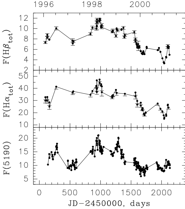
Fig. 3. The light curves of H\beta , H\alpha , and the continuum at the observed wavelength \lambda 5190 Å. The narrow components were not subtracted. Fluxes in lines are in units of 10^{-13} erg \text{cm}^{-2} \text{s}^{-1} , and in continuum in 10^{-15} erg \text{cm}^{-2} \text{s}^{-1} Å ^{-1} . The continuum is the “combined continuum” obtained from the spectra and photometric points in the V band in 1996–2001.
