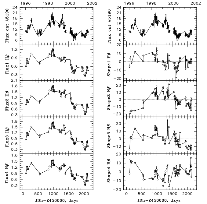
Fig. 9. Variations of the flux (left panel) and shapes (right panel) in different parts of the H\beta profile, and in the “combined” continuum at the observed wavelength \lambda 5190 Å. The radial velocity intervals of the profile segments: the H\beta 1 , H\alpha 1 set goes from -3000 \text{km s}^{-1} to -2000 \text{km s}^{-1} ; the H\beta 2 , H\alpha 2 set goes from -1500 \text{km s}^{-1} to -500 \text{km s}^{-1} ; the H\beta 3 , H\alpha 3 set goes from +500 \text{km s}^{-1} to +1500 \text{km s}^{-1} ; the H\beta 4 , H\alpha 4 set goes from +2000 \text{km s}^{-1} to +3000 \text{km s}^{-1} . The flux in the lines are given in units of 10^{-13} \text{erg cm}^{-2} \text{ s}^{-1} , and in the continuum are given in units of 10^{-15} \text{erg cm}^{-2} \text{ s}^{-1} \text{ Å}^{-1} . The shapes are in relative units (see Sect. 3.3.1).
