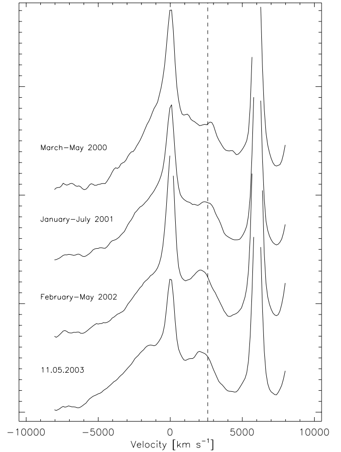
Fig. 7. Year-averaged normalized profiles of H \beta in 2000–2003. The vertical dashed line corresponds to a radial velocity +2600 km s ^{-1} . The abscissae give the radial velocities relative to the narrow component of H \beta . The profiles are shifted vertically by a constant value.
