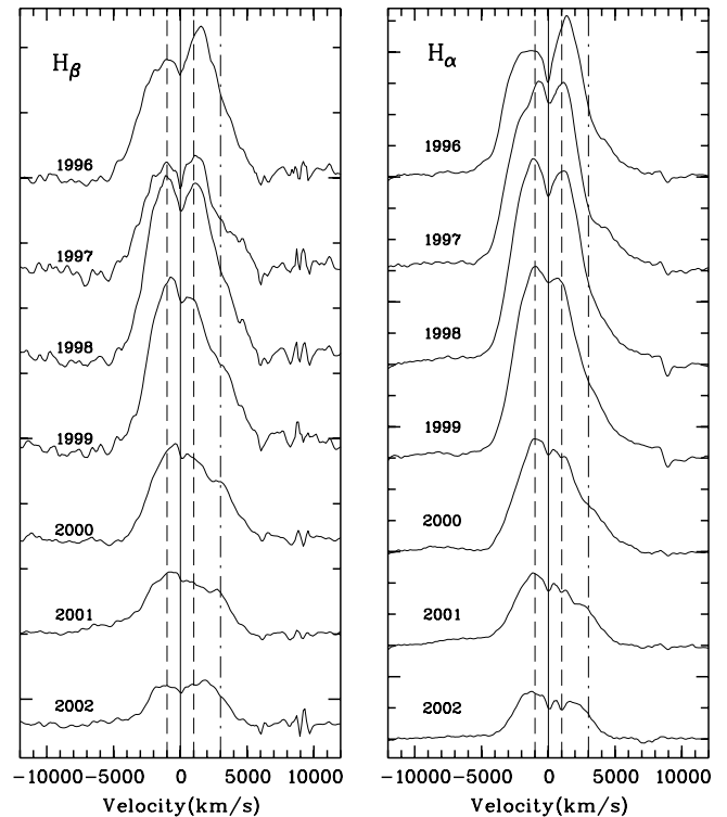
Fig. 8. Annual averages from 1996 to 2002 of the difference profiles of the broad H \beta (left panel) and H \alpha (right panel) lines. The vertical lines correspond to the radial velocities: dashed lines: \pm 1000 km s ^{-1} ; dash-dotted lines: \sim +3000 km s ^{-1} ; thin lines: 0 km s ^{-1} . The abscissae represent the radial velocities relative to the narrow component of H \beta and H \alpha . The ordinates give the relative fluxes. The profiles are shifted vertically by a constant value.
