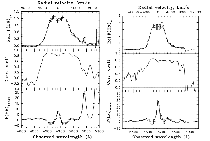
Fig. 4. The H\beta (left) and H\alpha (right) profile decomposition of the variable (top) and constant (bottom) components. The flux of the constant components is in units 10^{-15} erg \text{cm}^{-2} \text{s}^{-1} Å ^{-1} . For the variable components, the relative increment of the line flux when the continuum flux increases by an amount of 1 \times 10^{-15} erg \text{cm}^{-2} \text{s}^{-1} Å ^{-1} is shown. The correlation coefficient between the variable component of lines and the continuum flux at different wavelengths along the line profile is shown in the middle panels.
