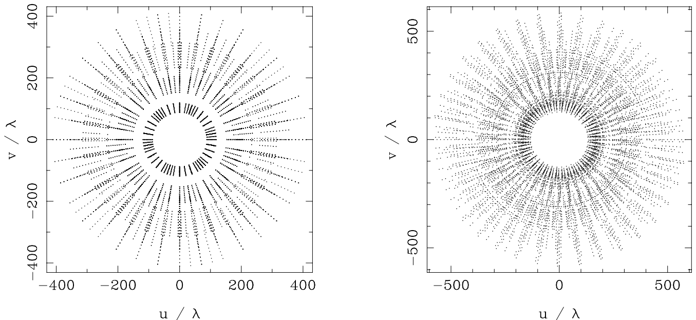
Figure 1. (u, v) coverage of the CBI1 (left) and CBI2 (right) in the configurations used for the observations of \zeta Oph on the left and LDN 1780 on the right. Axes are in units of wavelength ( \lambda ).
