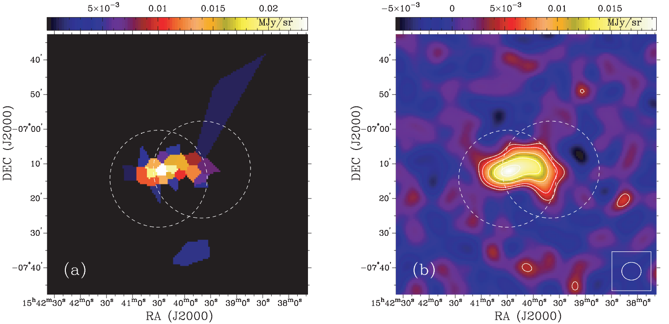
Figure 3. Left: Voronoi model of the visibilities of LDN 1780. This model has 55 polygons. Right: the convolution of the model in the left with the synthetic beam of the data, obtained using natural weights.
