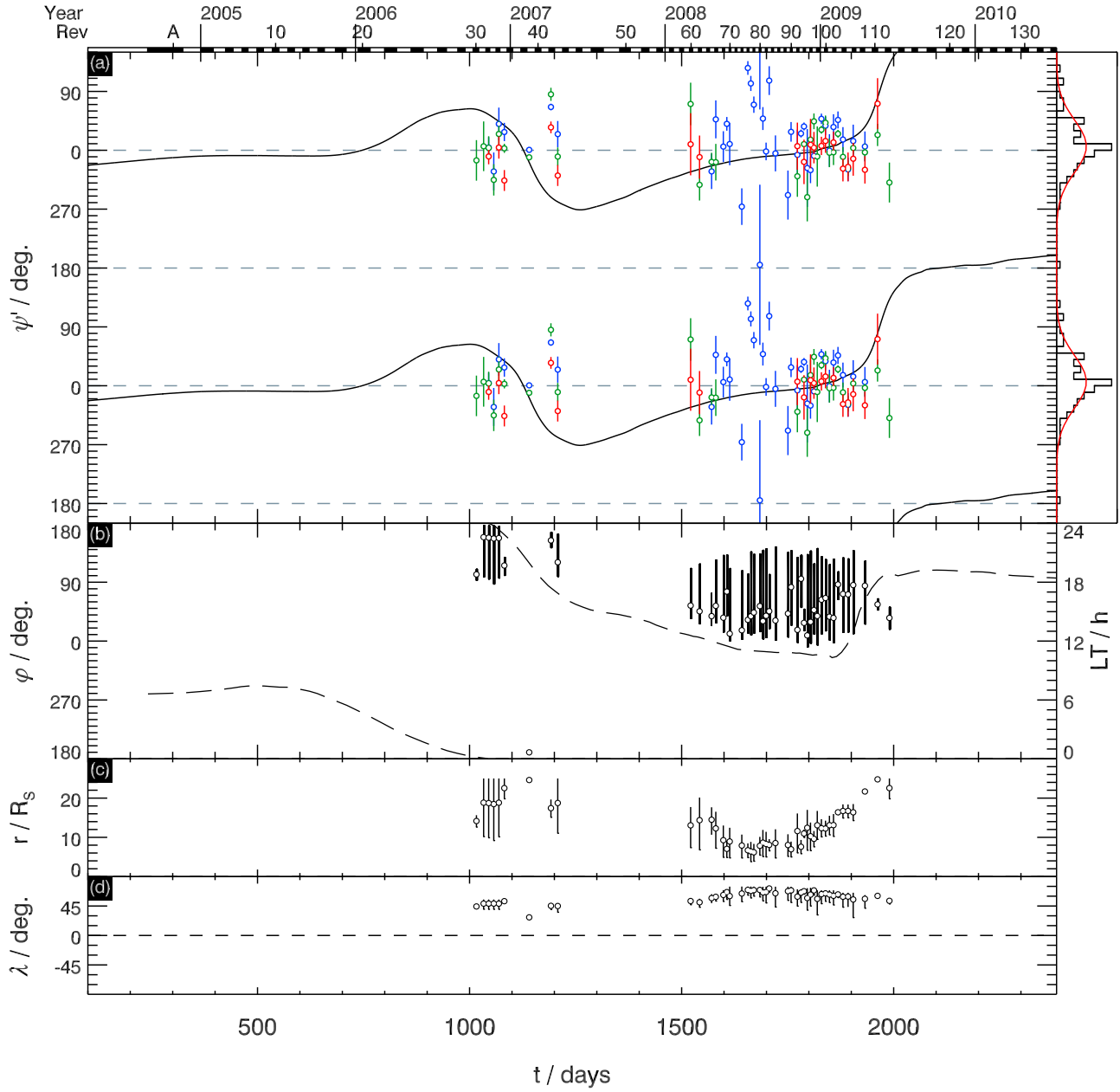
Figure 6. Northern period magnetic field phase data and related orbit parameters, in a format similar to that of Figures 5a–5d. The phases of the r field component are again shown as measured, while those of the \theta and \varphi components have been adjusted by the addition of 180^\circ and 90^\circ , respectively, to bring them to a common value.
