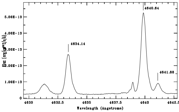
Fig. 14. The FEROS spectrum of the three N III lines close to \lambda 4640. The continuum has been scaled to that of STIS.
