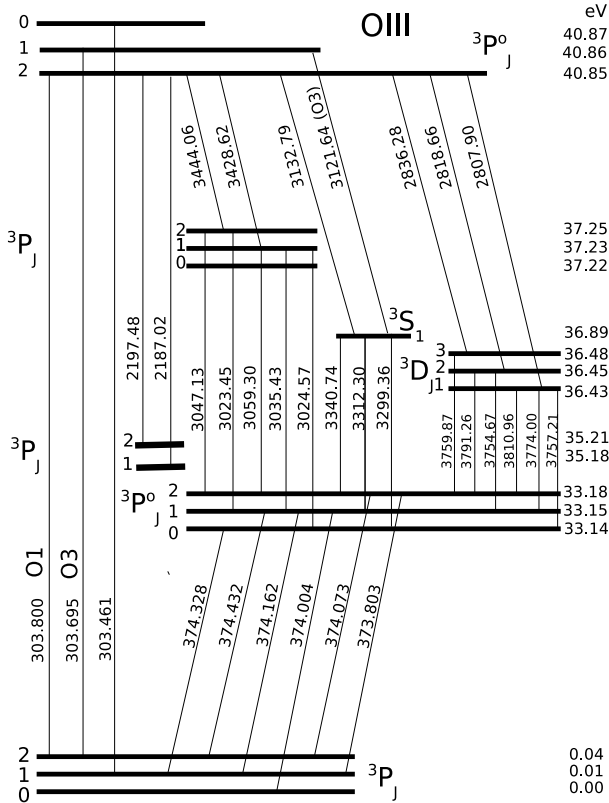
Fig. 6. A partial Grotrian diagram of O III that includes the most relevant O1 transitions and the \lambda 3121.64 line belonging to the O3 process. The level's configuration can be read from Table 3. The y -axis is not scaled linearly.
