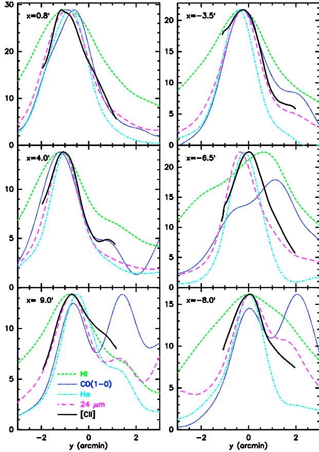
Fig. 3. Cuts across the spiral arm in [CII], CO(1–0), HI, H \alpha , and the 24 \mu\text{m} continuum. The x position refers to the horizontal axis position of the cut on the maps in Fig. 2. The maxima of all the cuts have been normalized to the maximum of the cut in the [CII] image. The units of the y -axis are those of the cut in the [CII] image ( 10^{-20} \text{ W cm}^{-2} ).
