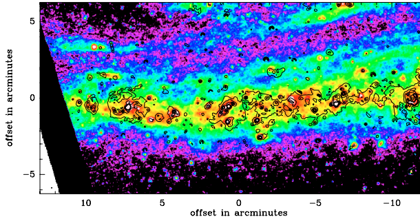
Fig. 4. Spitzer 24 \mu\text{m} image with H \alpha contours superposed. Note the excellent correspondance despite the inclination of M 31 and the difference in extinction between the two images.
