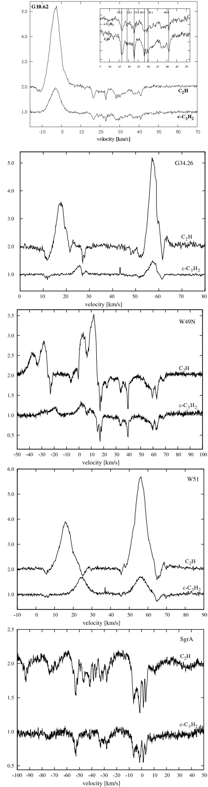
Fig. 1. Spectra obtained with the IRAM-30 m telescope. The velocity scale is given relative to the Local Standard of Rest (LSR). The spectra have been normalized by dividing the individual measurements by the source continuum intensities. The CCH spectra have been offset for clarity. Except for G10.6, the two strongest CCH hyperfine components at 87.317 and 87.329 GHz are shown. The emission line shifted by -31.6 \text{ km s}^{-1} from c-C 3 H 2 is the HCS + J = 2-1 transition at 85.347 GHz. An inset showing the velocities of the absorption features is presented for G10.62.
