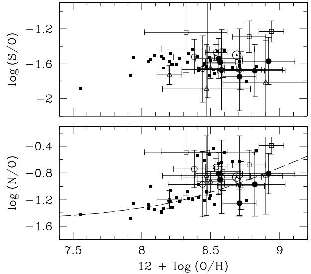
Fig. 18. Same as Fig. 17, but including only nebulae from the VLT sample where the electron temperature has been computed from the availability of at least one of the [\text{N II}] \lambda 5755 and [\text{S III}] \lambda 6312 auroral lines (objects marked by asterisks in Table 12). The dashed line represents a simple model, in which a primary nitrogen component is superposed on a secondary component, which is proportional to O/H.
