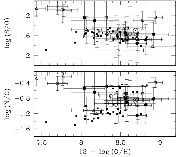
Fig. 17. The S/O (top) and N/O (bottom) abundance ratio trends with O/H for all objects in Table 12. A comparison sample, drawn from Garnett et al. (1997, NGC 2403), Kennicutt et al. (2003, M 101) and Bresolin et al. (2004, M 51), is shown by small full square symbols. The solar values, indicated by the \odot symbol, are taken from Lodders (2003).
