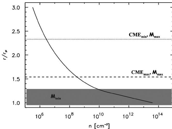
Fig. 3. Neutral hydrogen density profile of the upper atmosphere under hydrodynamic conditions of HD209458b as a function of planetocentric distance in units of planetary radii. The dotted and dashed lines mark the magnetopause stand-off distance corresponding to the minimum and maximum CME plasma densities, respectively, and the maximum expected magnetic moment \mathcal{M}_{\text{max}} = 0.1 \mathcal{M}_{\text{Jup}} . In the case of the minimum expected magnetic moment of HD209458b \mathcal{M}_{\text{min}} = 0.005 \mathcal{M}_{\text{Jup}} , the magnetopause stand-off distances would lay below the visual planetary radius at about 0.56\text{--}0.8r_{\text{pl}} . Since at deep atmospheric levels the neutral gas density is very high, one can expect that the CME plasma flow will be deflected around the planet at somewhat higher altitudes which are shown as a shaded area.
