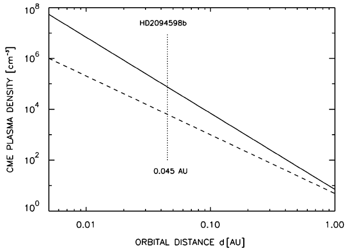
Fig. 1. Minimum (dashed-line) and maximum (solid-line) CME and ICME plasma density as a function of orbital distance.
