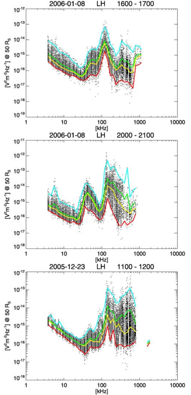
Figure 6. Variability of the SKR ‘classic’ spectrum where only one maximum is observed at low (between 40 kHz and 200 kHz) and high (between 100 kHz and 900 kHz) as it is shown in the top and bottom panels, respectively. Sometimes both maxima are observed (middle panel).
